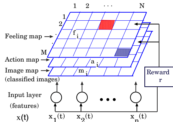
Fig. 1 Structure of a hierarchical SOM.
